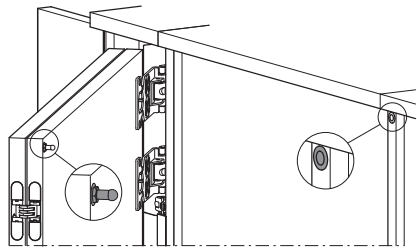
Application with pin and sleeve
