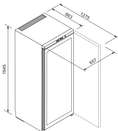
Installation Diagram
