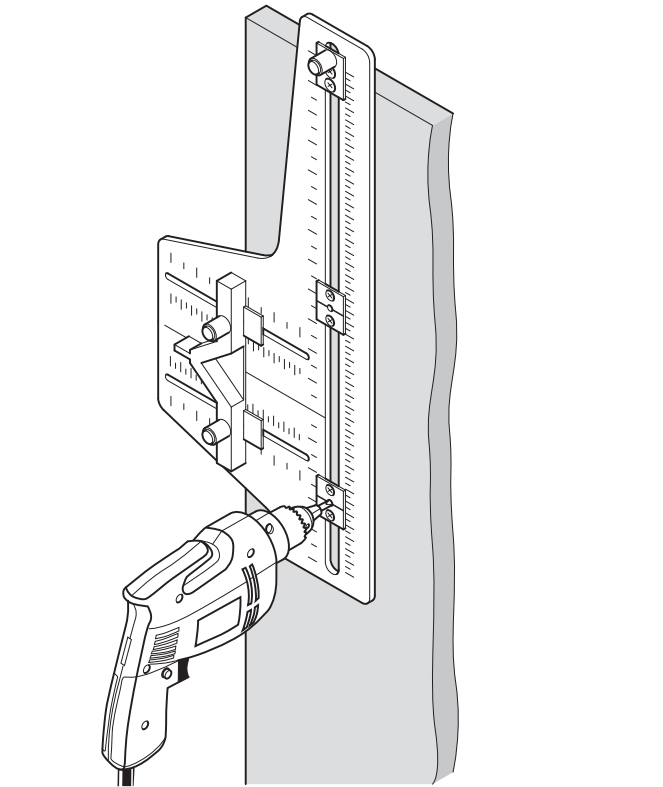
Drilling on doors and flaps
