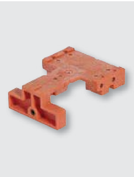
Fixing position of the snap-in coupling Hook position of the drawer rail
