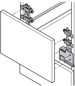
Drawer front processing
