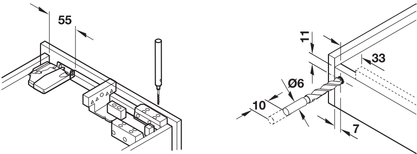
Fixing position of the snap-in coupling Hook position of the drawer rail
